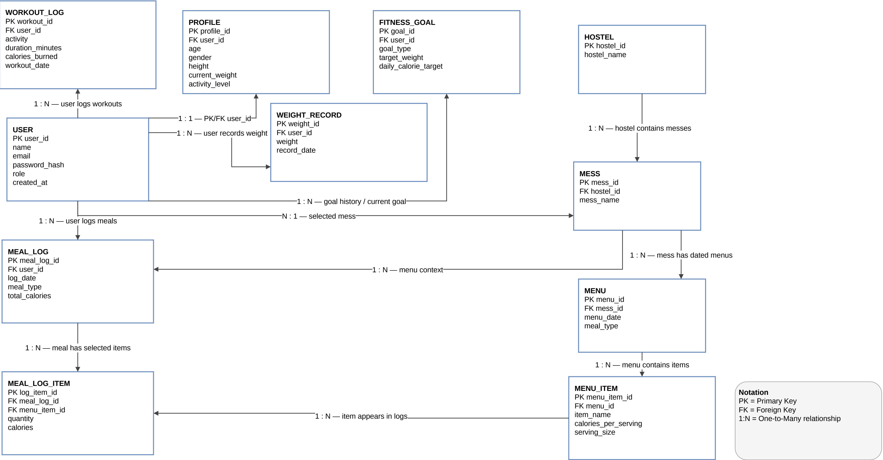
ER Diagram — HostelFit: Mess Calorie & Workout Tracker
